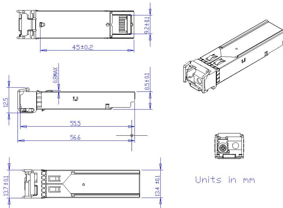
Figure2 Mechanical Outline
