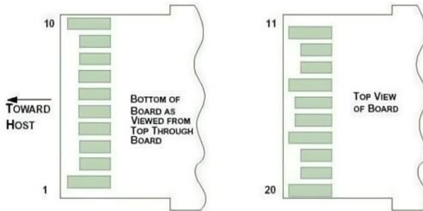
Figure 2: MSA Compliant Connector
