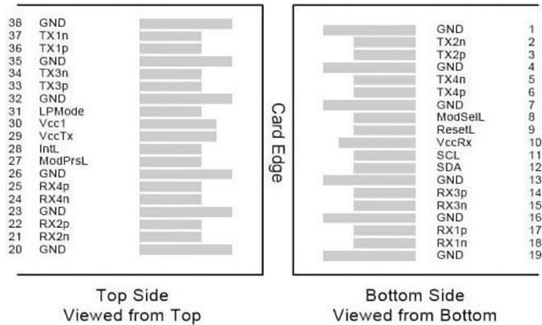
Figure 1: MSA Compliant Connector
