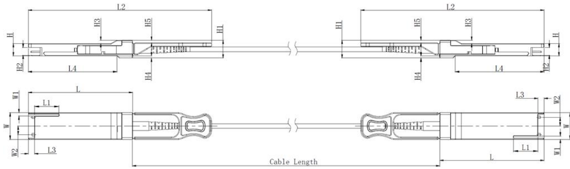
Figure 4 Mechanical Diagram
