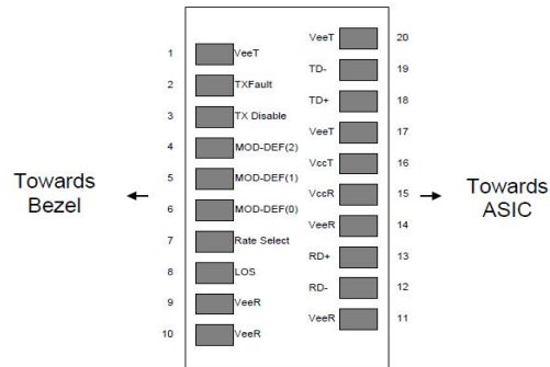
Figure 1 Pin view
