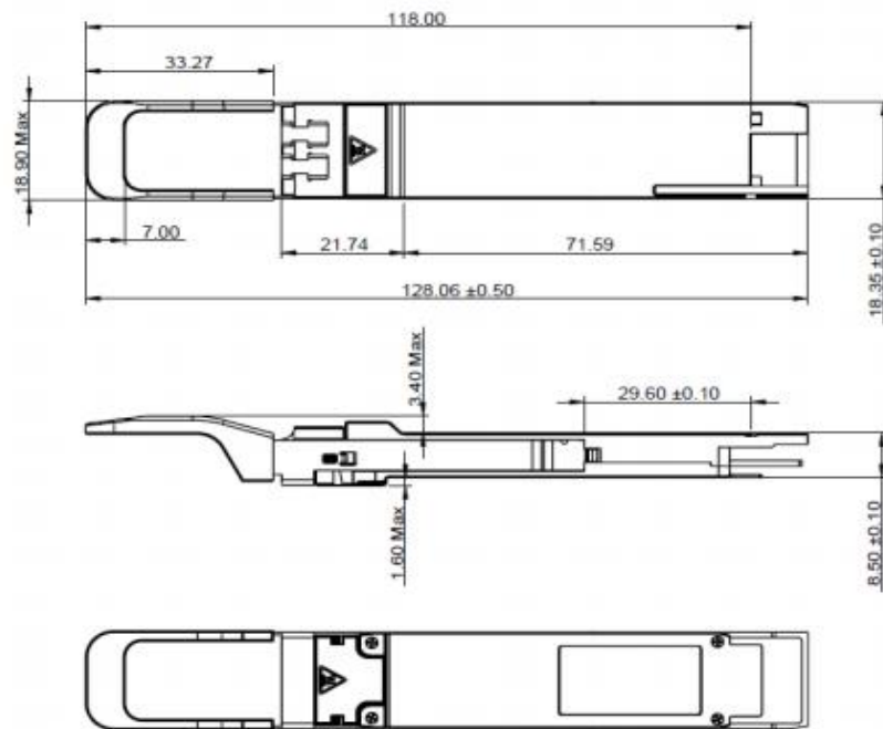
Figure4 Mechanical Outline
