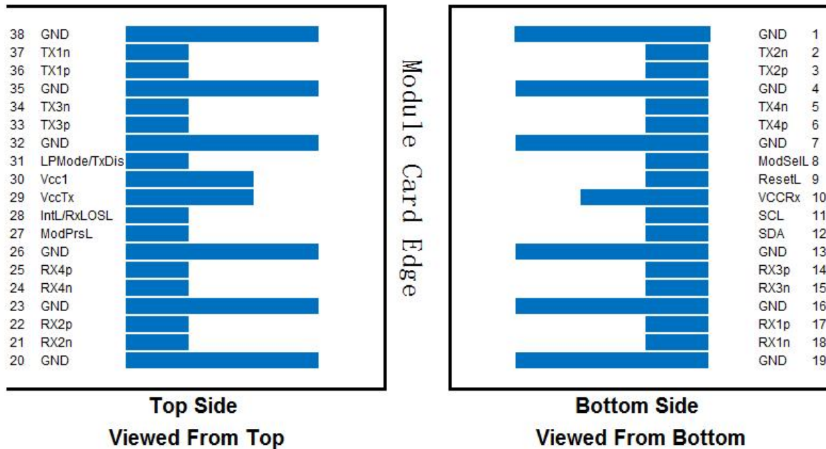
Figure 2 Pin view
