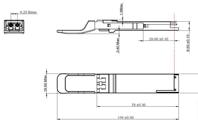
Figure 4 Mechanical Outline
