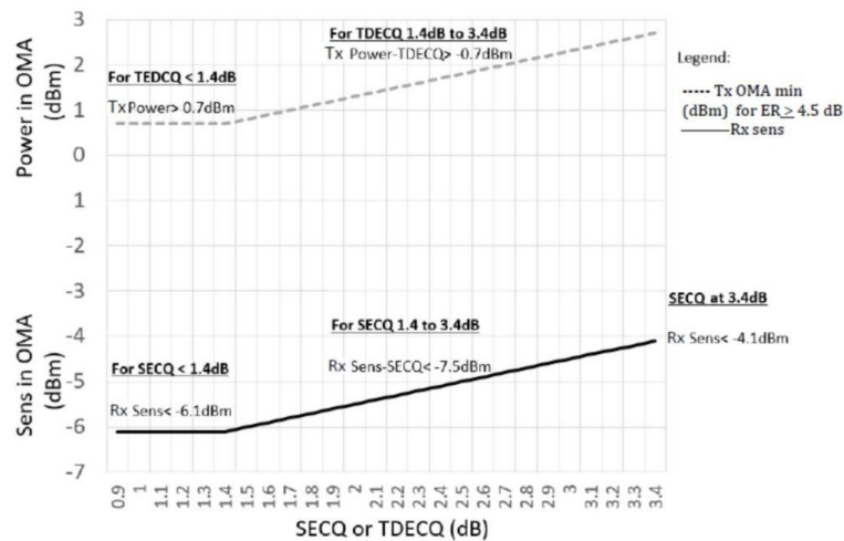
Figure 1 Illustration of Receiver Sensitivity Mask for 100G-LR
