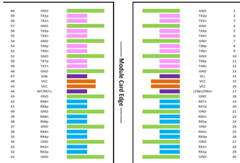
Figure 1 MSA Compliant Connector
