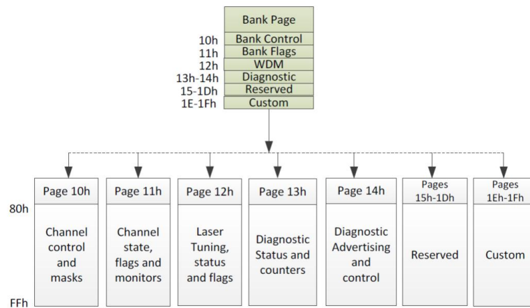
Figure 2 CMIS Module Memory Map
