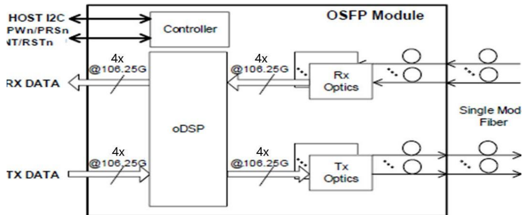
Figure 4 Block Diagram of Transceiver
