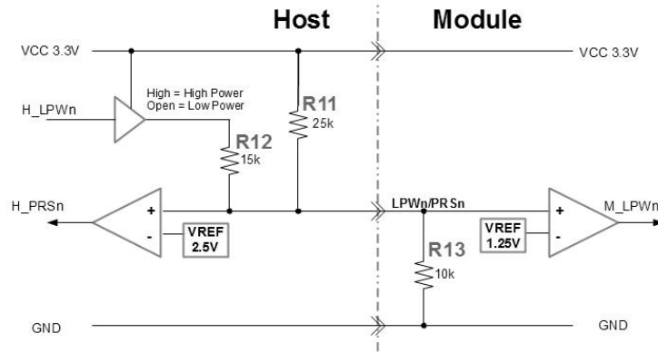
Figure2 INT/RSTn circuit
