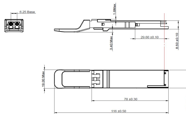
Figure 4 Mechanical Outline
