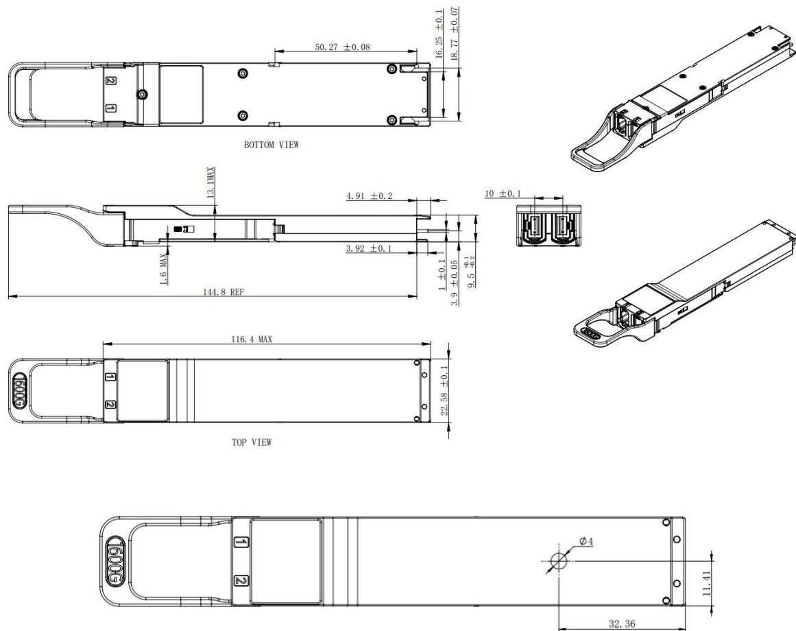
Figure 8 Riding HS Package Outline
