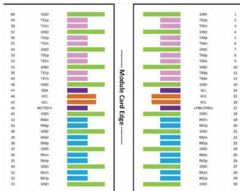
Figure 1 MSA Compliant Connector
