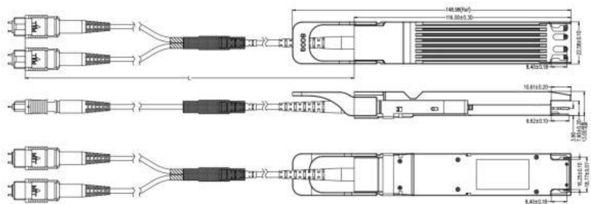
Figure5 Package dimensions (male)
