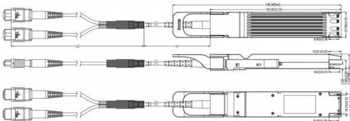
Figure4 Package dimensions (female)
